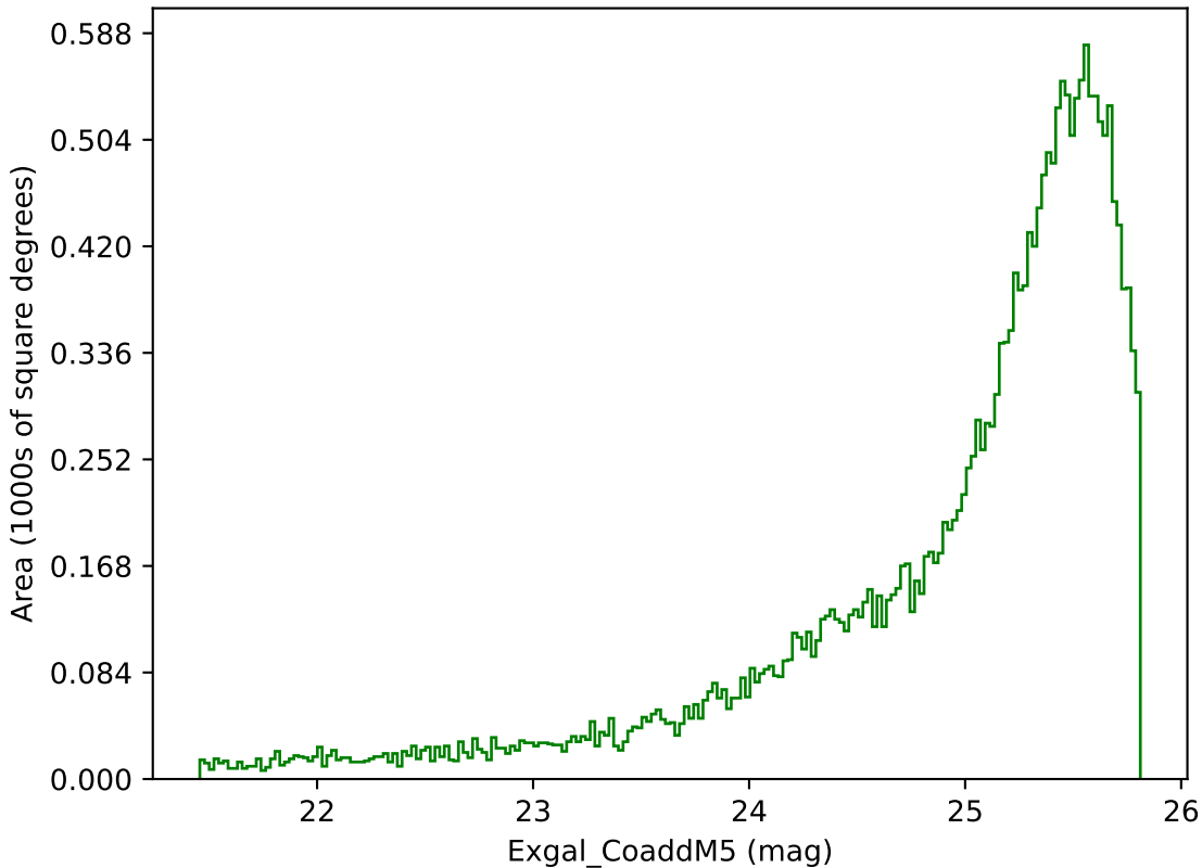
ddf_loaded_fl1_v3.4_10yrs Yr 1 g band: Exgal_CoaddM5
