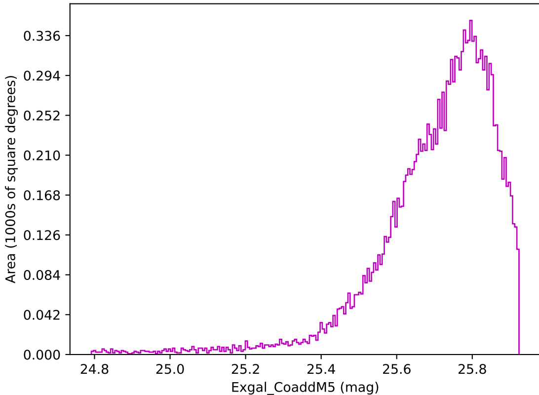
ddf_loaded_fl1_v3.4_10yrs WFD z band: Exgal_CoaddM5
