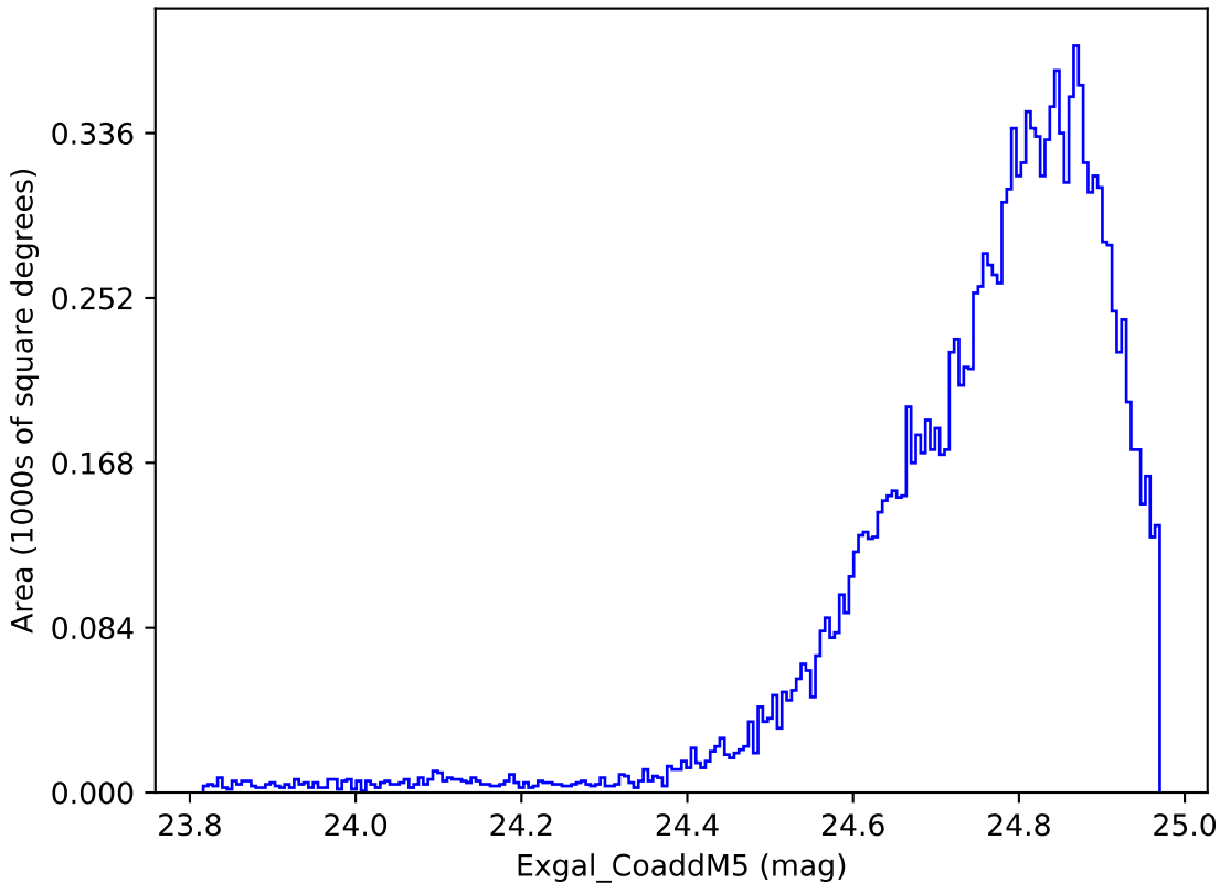
ddf_loaded_fl1_v3.4_10yrs WFD y band: Exgal_CoaddM5
