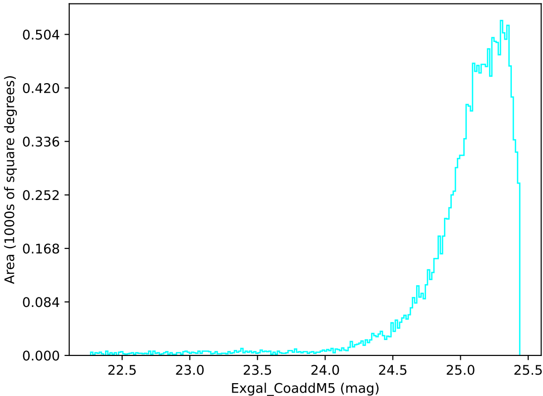
ddf_loaded_fl1_v3.4_10yrs WFD u band: Exgal_CoaddM5
