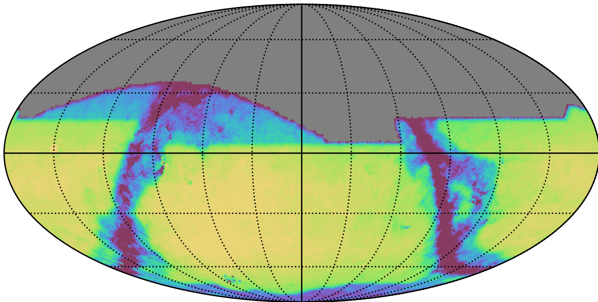
ddf_loaded_fl1_v3.4_10yrs All sky z band: Exgal_CoaddM5
