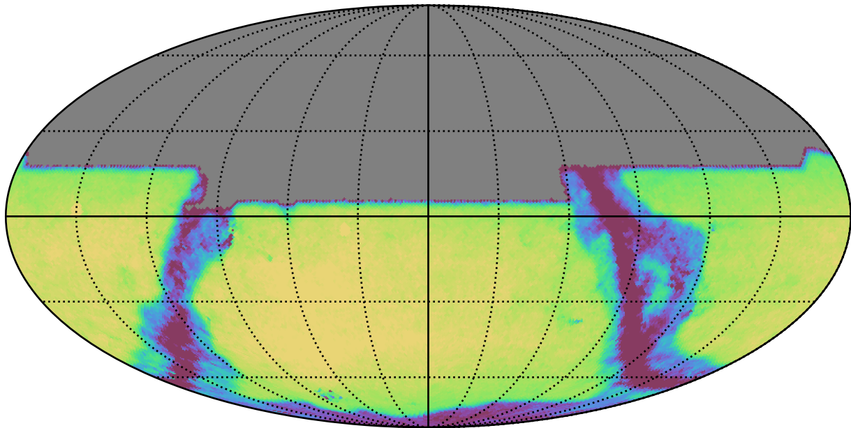
ddf_loaded_fl1_v3.4_10yrs All sky y band: Exgal_CoaddM5
