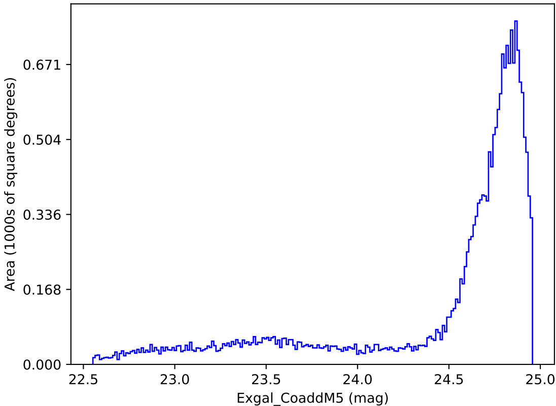
ddf_loaded_fl1_v3.4_10yrs All sky y band: Exgal_CoaddM5
