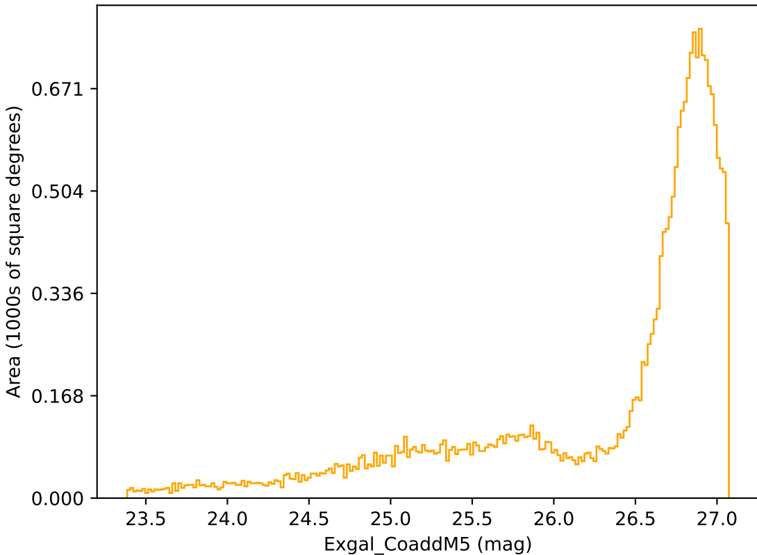
ddf_loaded_fl1_v3.4_10yrs All sky r band: Exgal_CoaddM5
