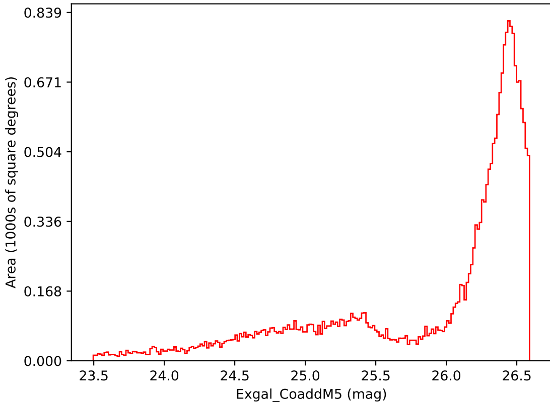
ddf_loaded_fl1_v3.4_10yrs All sky i band: Exgal_CoaddM5
