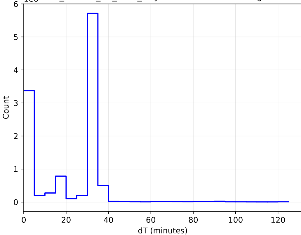
1e6 ddf_loaded_fl1_v3.4_10yrs WFD: DeltaT Histogram
