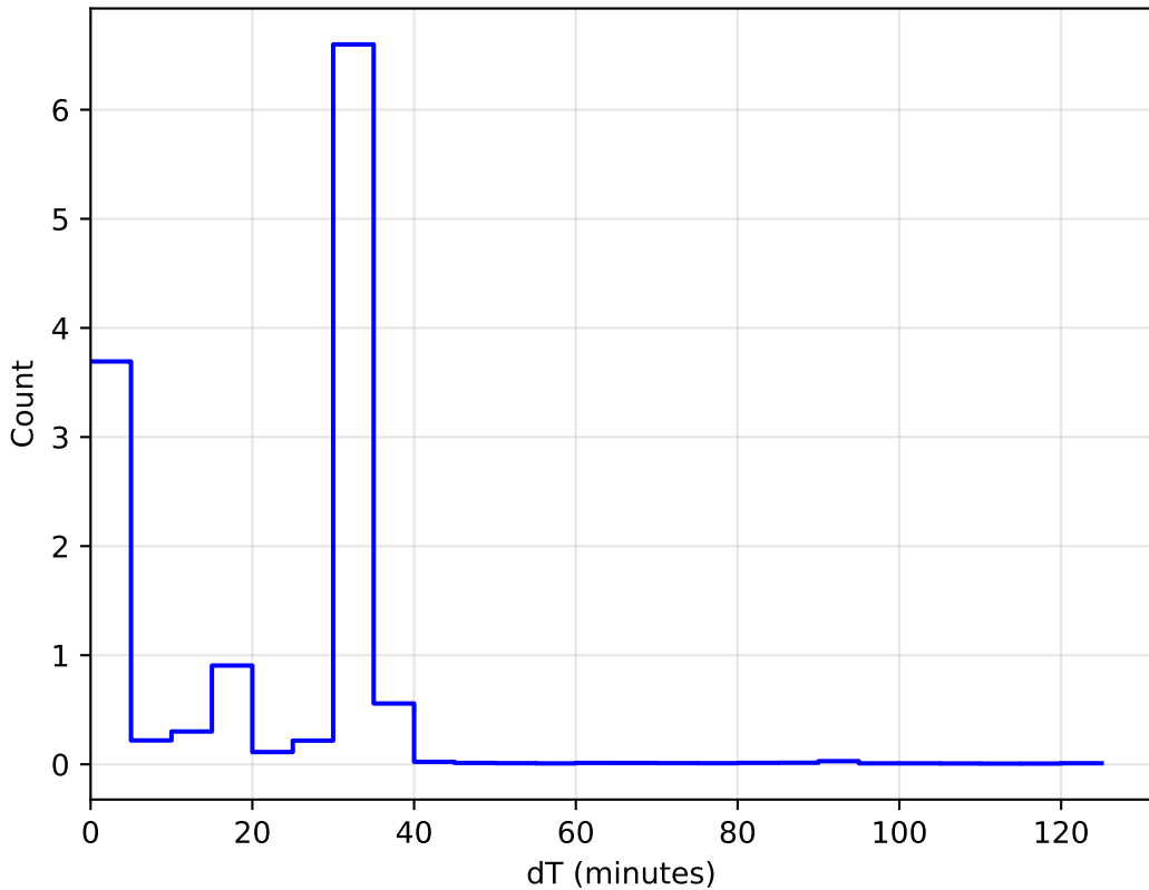
1e6 ddf_loaded_fl1_v3.4_10yrs All sky: DeltaT Histogram
