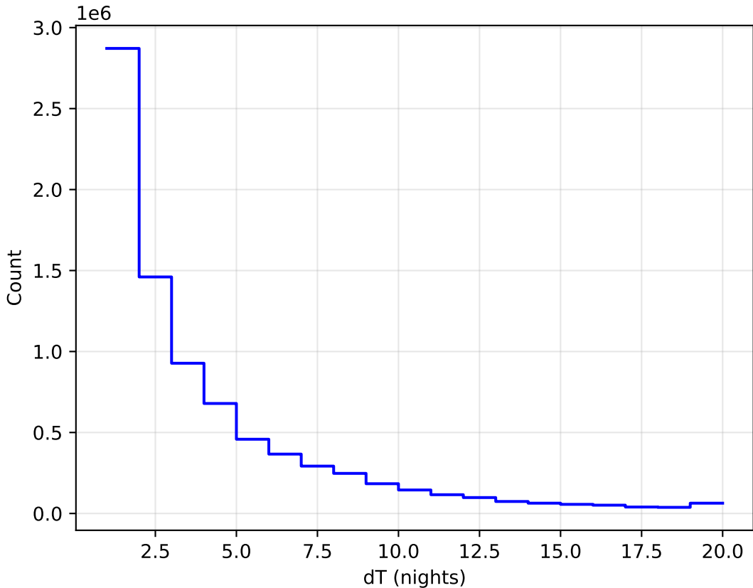
ddf_loaded_fl1_v3.4_10yrs WFD all bands: DeltaNight Histogram
