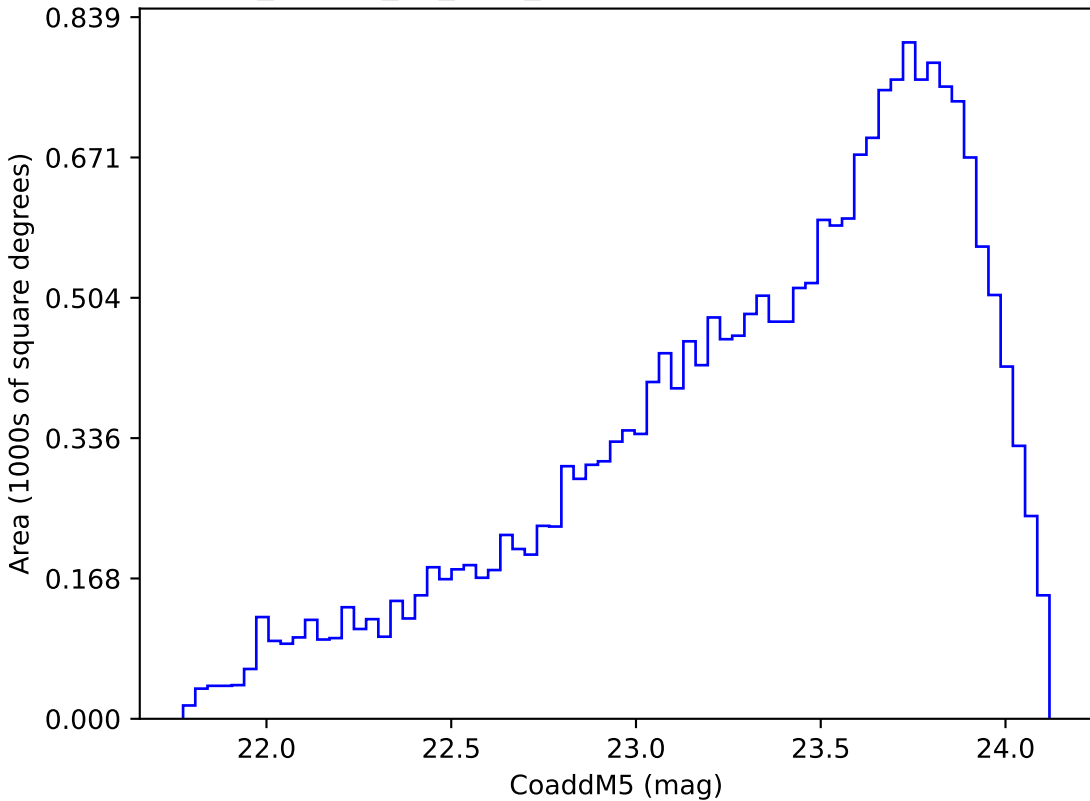
ddf_loaded_fl1_v3.4_10yrs Yr 3-4 y band: CoaddM5
