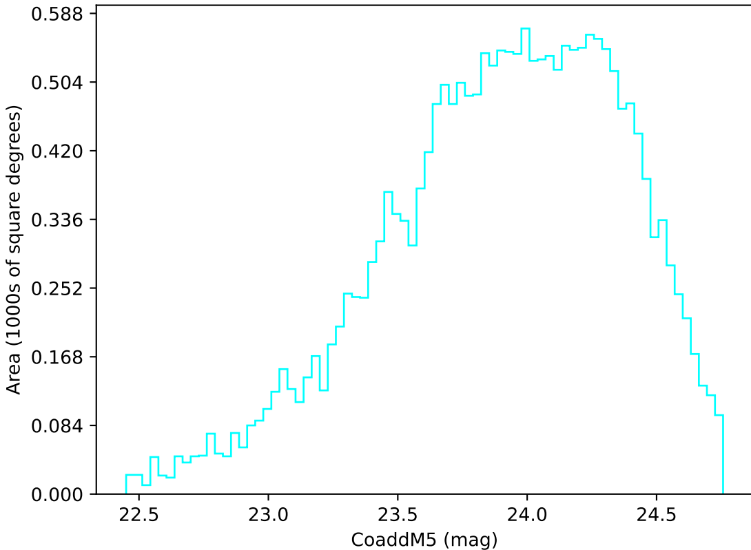
ddf_loaded_fl1_v3.4_10yrs Yr 3-4 u band: CoaddM5
