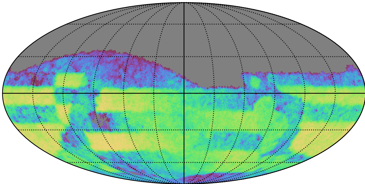
ddf_loaded_fl1_v3.4_10yrs Yr 3-4 i band: CoaddM5
