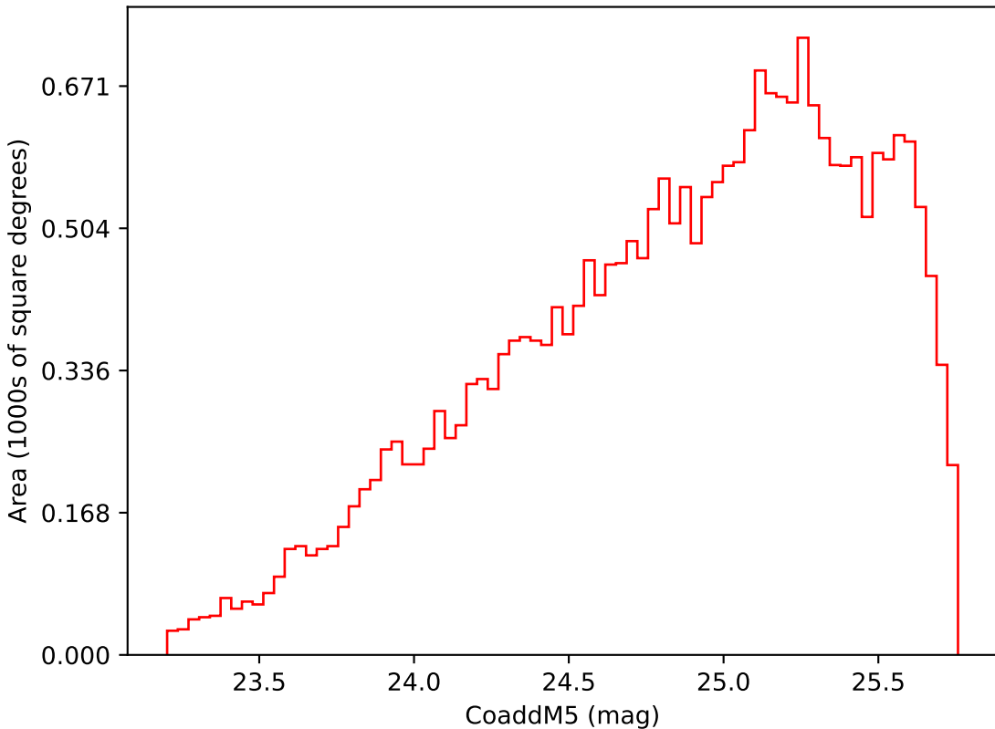
ddf_loaded_fl1_v3.4_10yrs Yr 3-4 i band: CoaddM5
