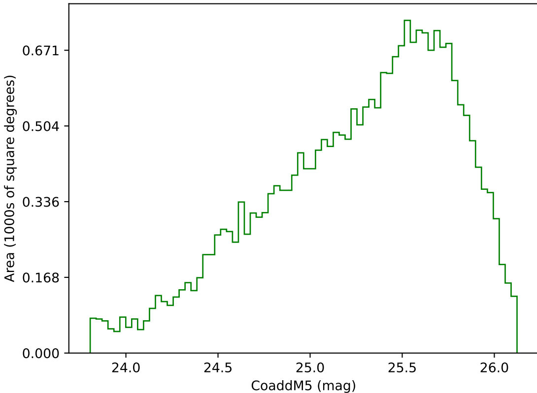
ddf_loaded_fl1_v3.4_10yrs Yr 3-4 g band: CoaddM5
