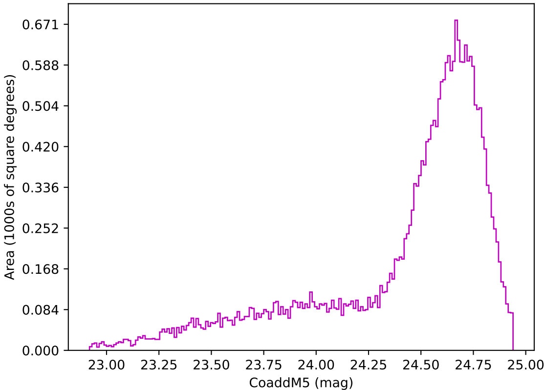
ddf_loaded_fl1_v3.4_10yrs Yr 1 z band: CoaddM5
