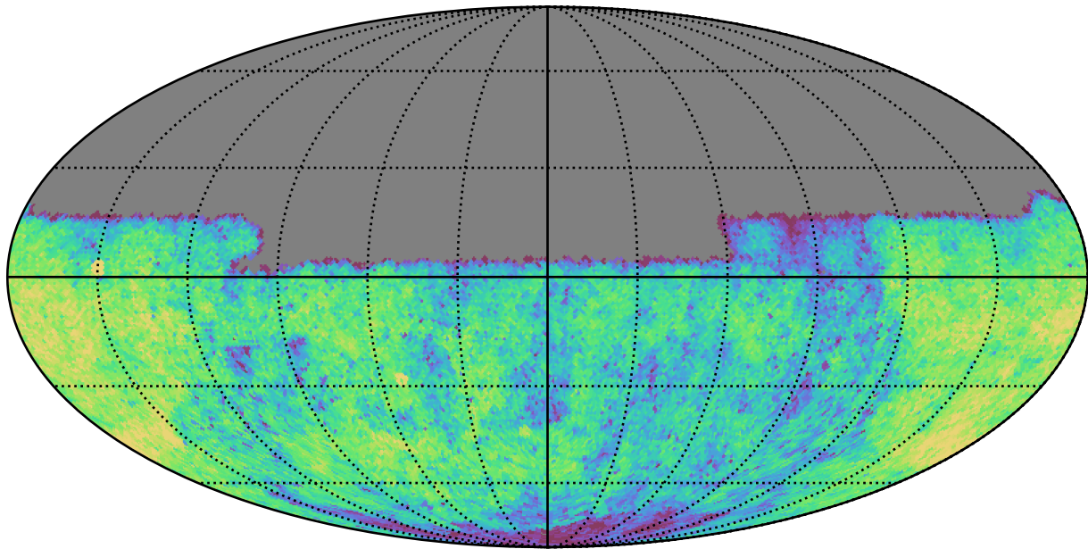
ddf_loaded_fl1_v3.4_10yrs Yr 1 u band: CoaddM5
