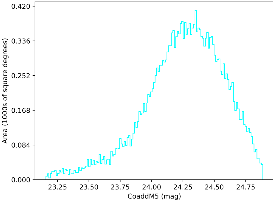
ddf_loaded_fl1_v3.4_10yrs Yr 1 u band: CoaddM5
