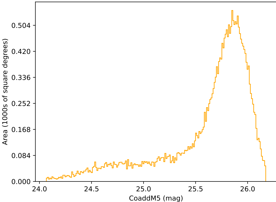
ddf_loaded_fl1_v3.4_10yrs Yr 1 r band: CoaddM5
