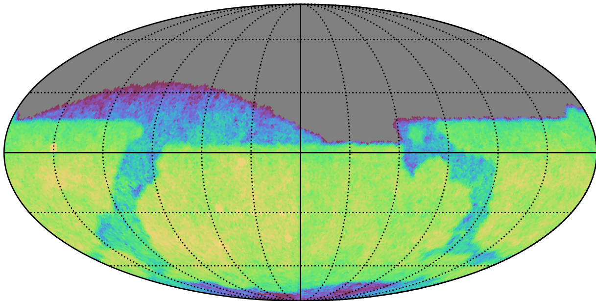
ddf_loaded_fl1_v3.4_10yrs Yr 1 i band: CoaddM5
