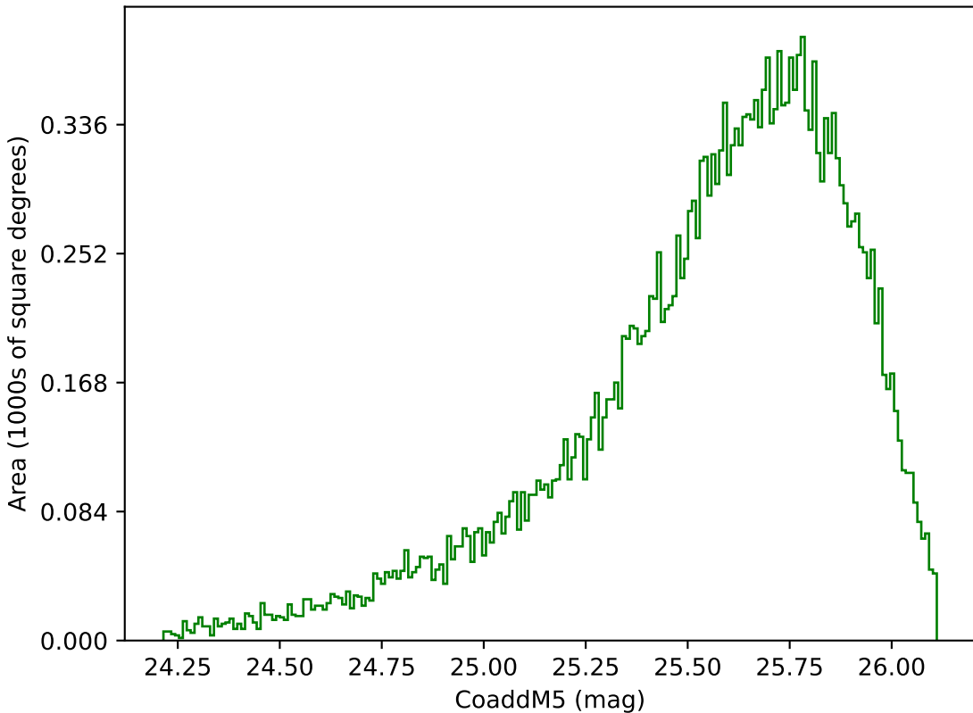
ddf_loaded_fl1_v3.4_10yrs Yr 1 g band: CoaddM5
