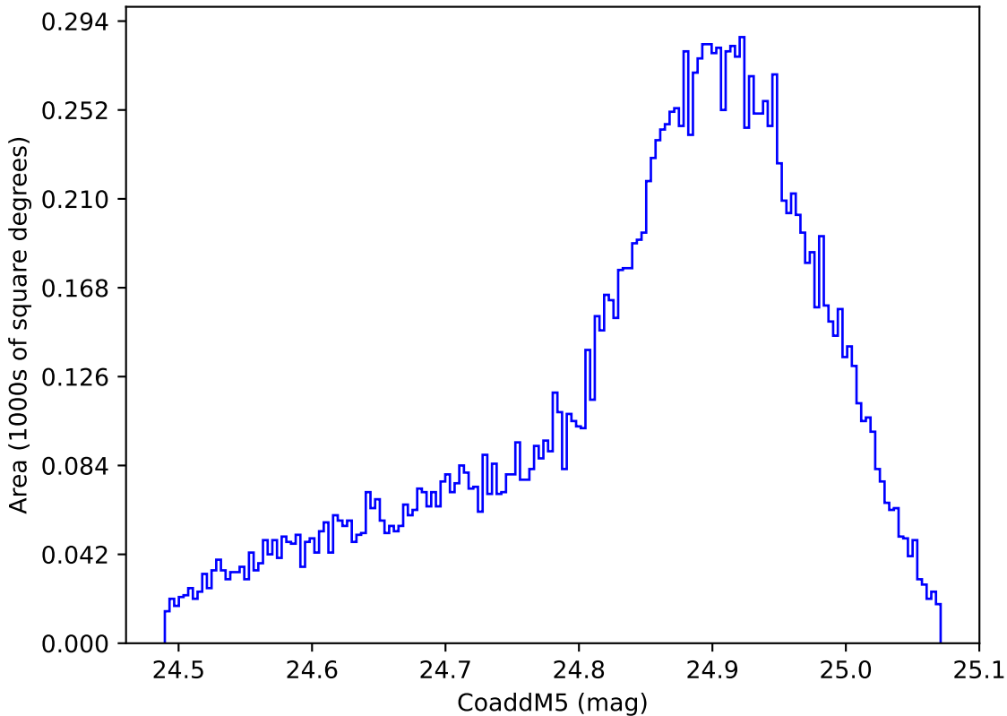
ddf_loaded_fl1_v3.4_10yrs WFD y band: CoaddM5
