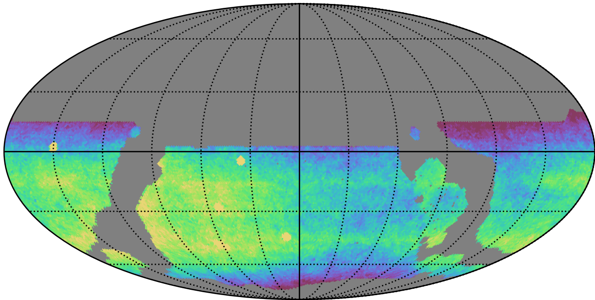
ddf_loaded_fl1_v3.4_10yrs WFD r band: CoaddM5
