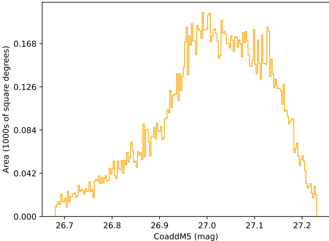
ddf_loaded_fl1_v3.4_10yrs WFD r band: CoaddM5
