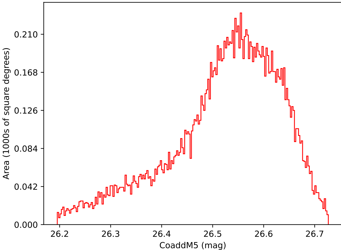
ddf_loaded_fl1_v3.4_10yrs WFD i band: CoaddM5
