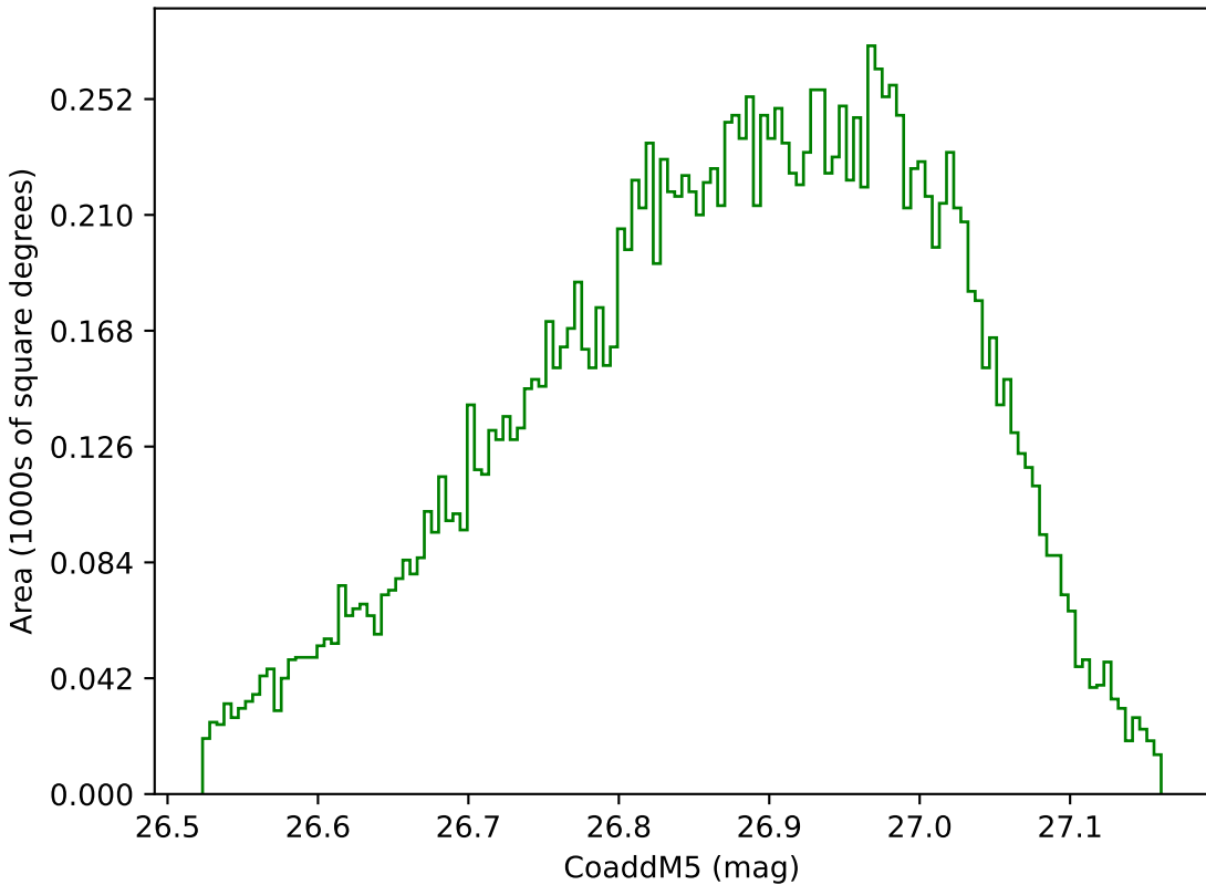
ddf_loaded_fl1_v3.4_10yrs WFD g band: CoaddM5
