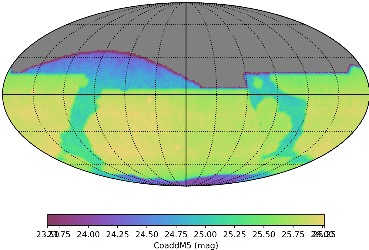
ddf_loaded_fl1_v3.4_10yrs All sky z band: CoaddM5
