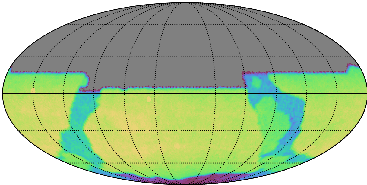
ddf_loaded_fl1_v3.4_10yrs All sky y band: CoaddM5
