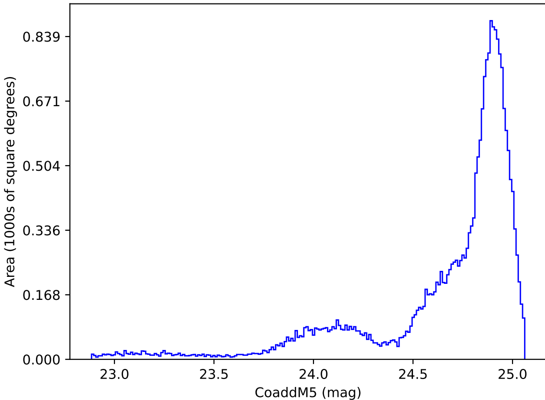
ddf_loaded_fl1_v3.4_10yrs All sky y band: CoaddM5
