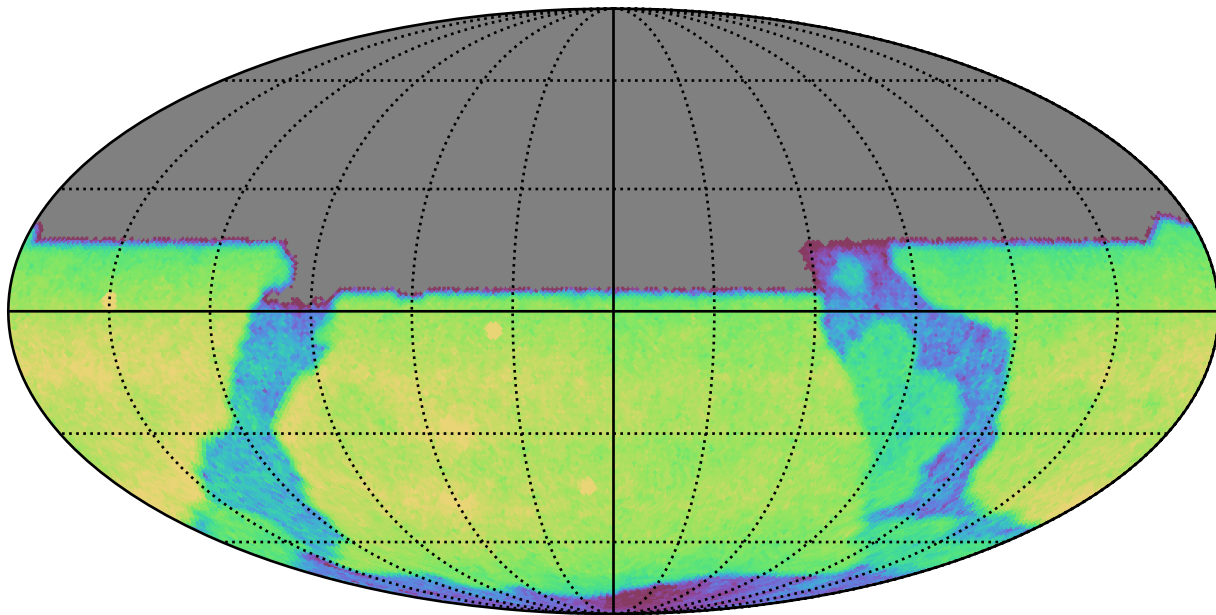
ddf_loaded_fl1_v3.4_10yrs All sky u band: CoaddM5
