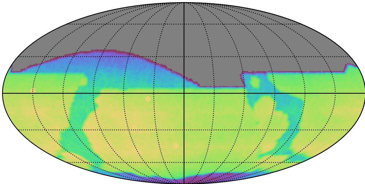
ddf_loaded_fl1_v3.4_10yrs All sky r band: CoaddM5
