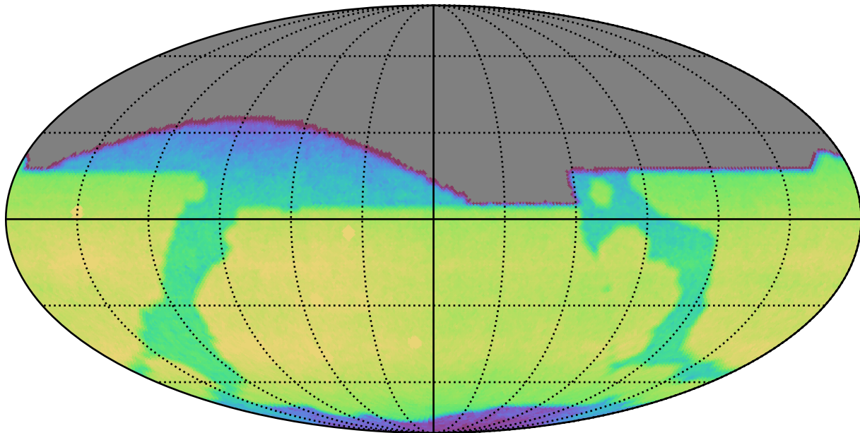
ddf_loaded_fl1_v3.4_10yrs All sky i band: CoaddM5
