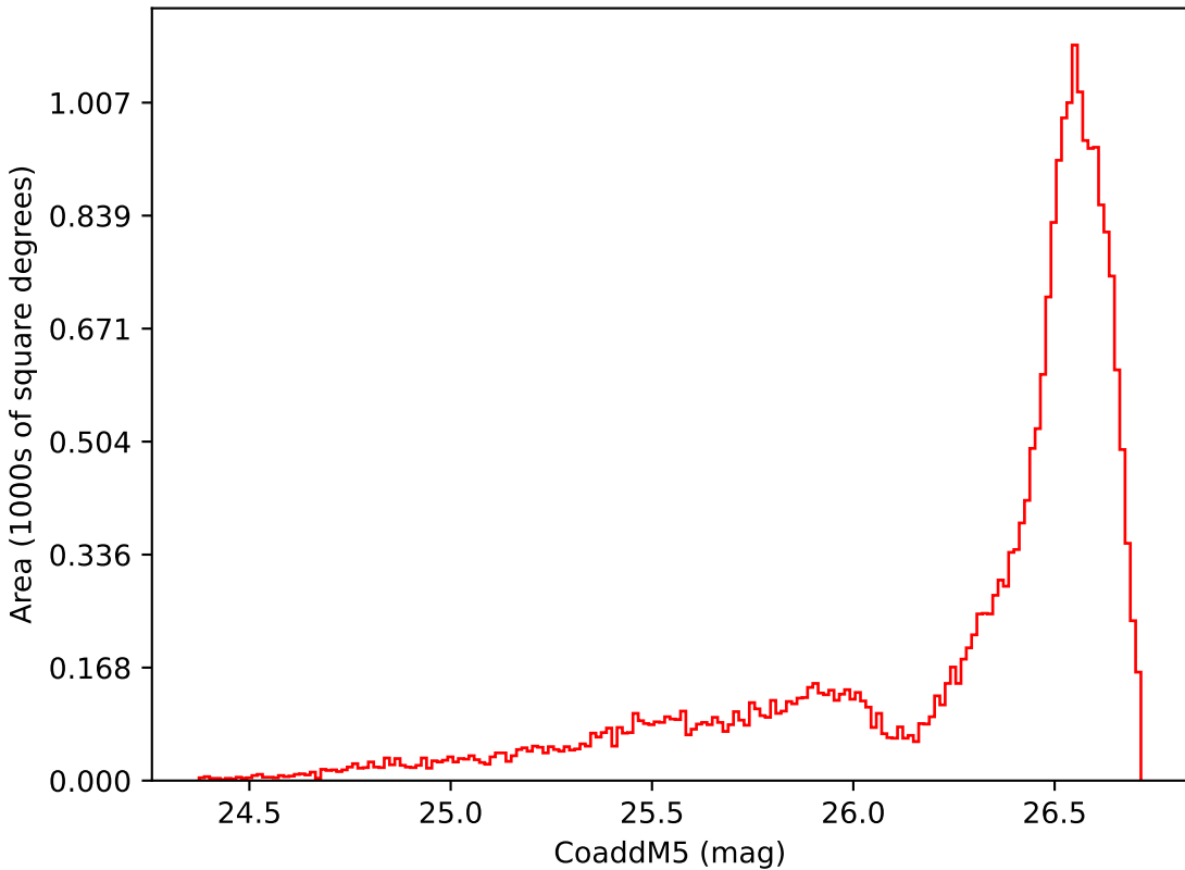
ddf_loaded_fl1_v3.4_10yrs All sky i band: CoaddM5
