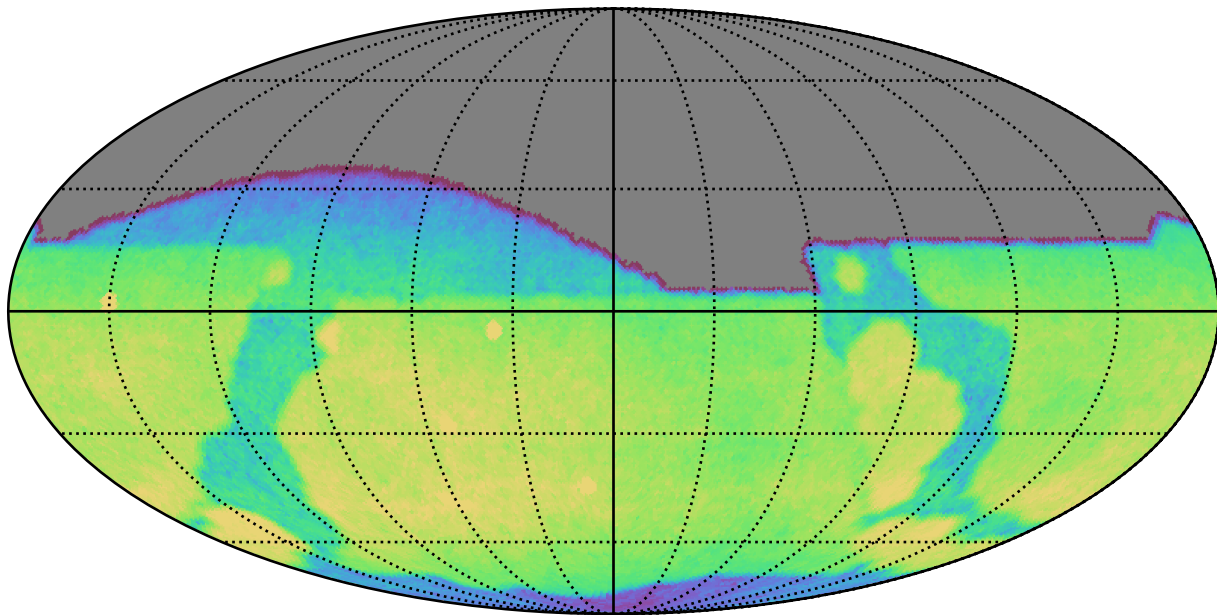
ddf_loaded_fl1_v3.4_10yrs All sky g band: CoaddM5
