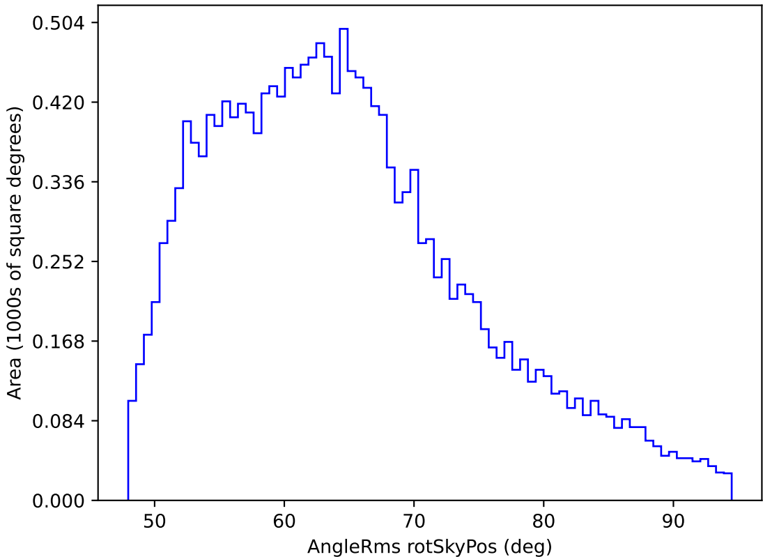
ddf_loaded_fl1_v3.4_10yrs WFD z band: AngleRms rotSkyPos
