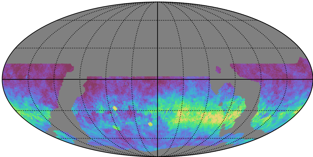
ddf_loaded_fl1_v3.4_10yrs WFD y band: AngleRms rotSkyPos
