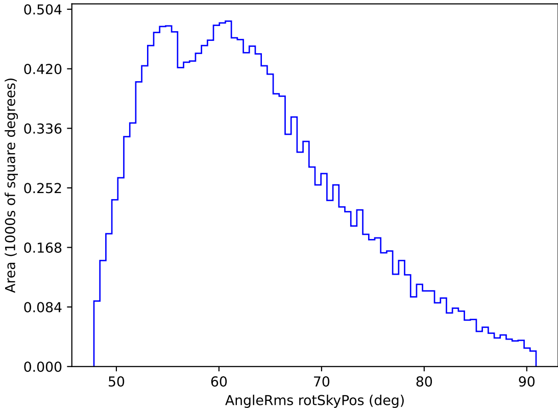
ddf_loaded_fl1_v3.4_10yrs WFD y band: AngleRms rotSkyPos
