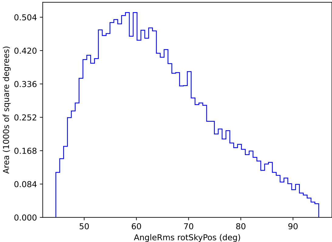
ddf_loaded_fl1_v3.4_10yrs WFD u band: AngleRms rotSkyPos
