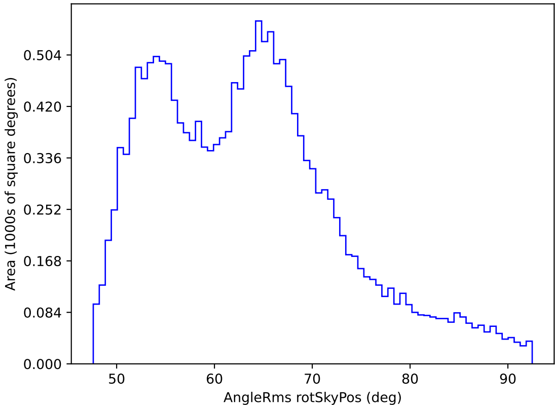
ddf_loaded_fl1_v3.4_10yrs WFD i band: AngleRms rotSkyPos
