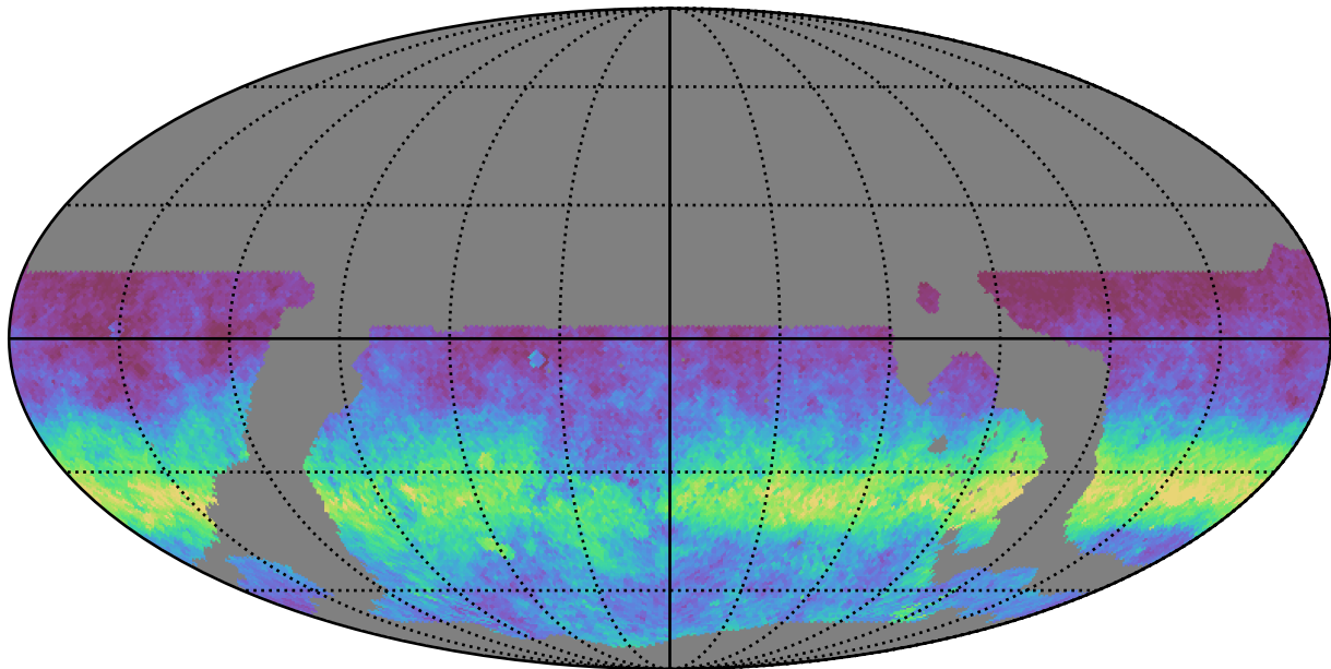
ddf_loaded_fl1_v3.4_10yrs WFD g band: AngleRms rotSkyPos
