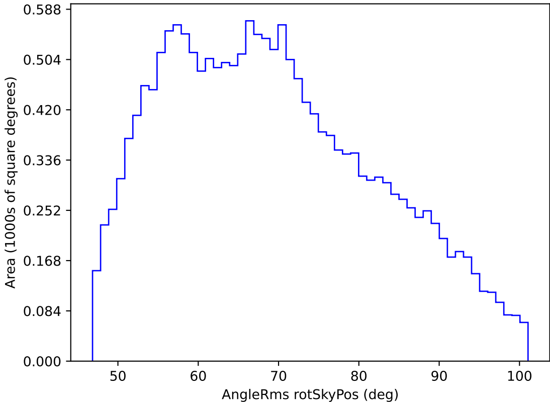
ddf_loaded_fl1_v3.4_10yrs WFD g band: AngleRms rotSkyPos
