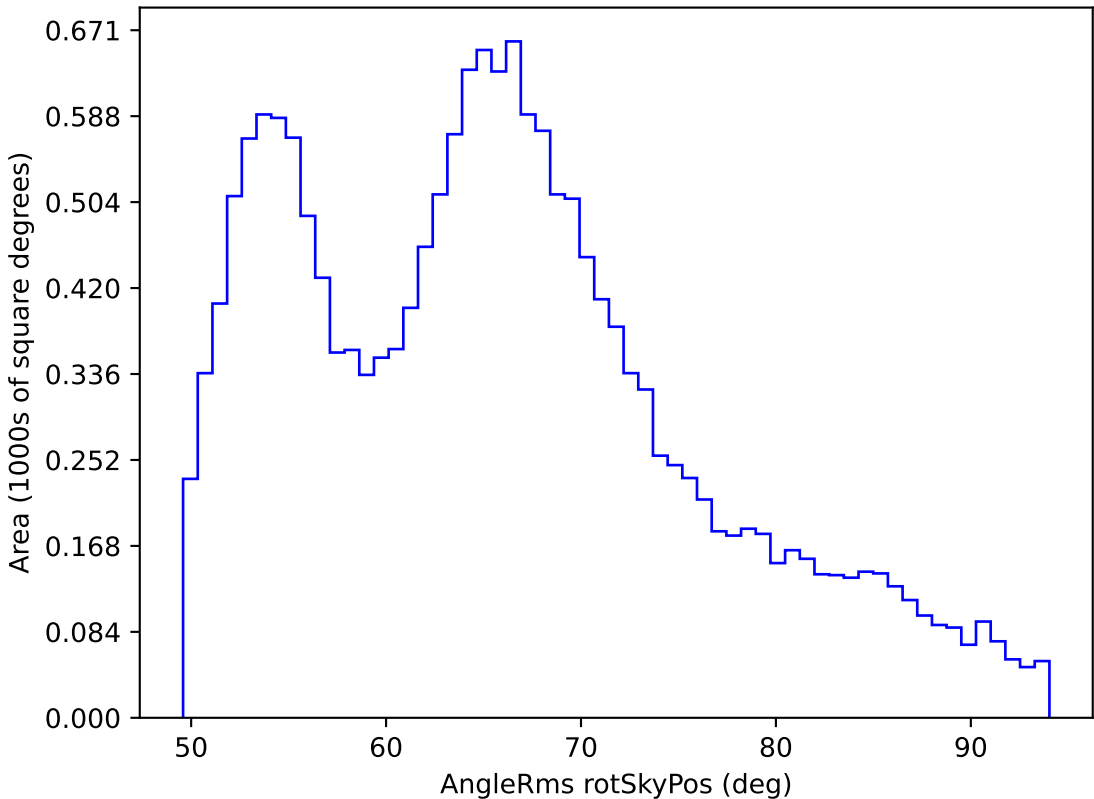
ddf_loaded_fl1_v3.4_10yrs WFD all bands: AngleRms rotSkyPos
