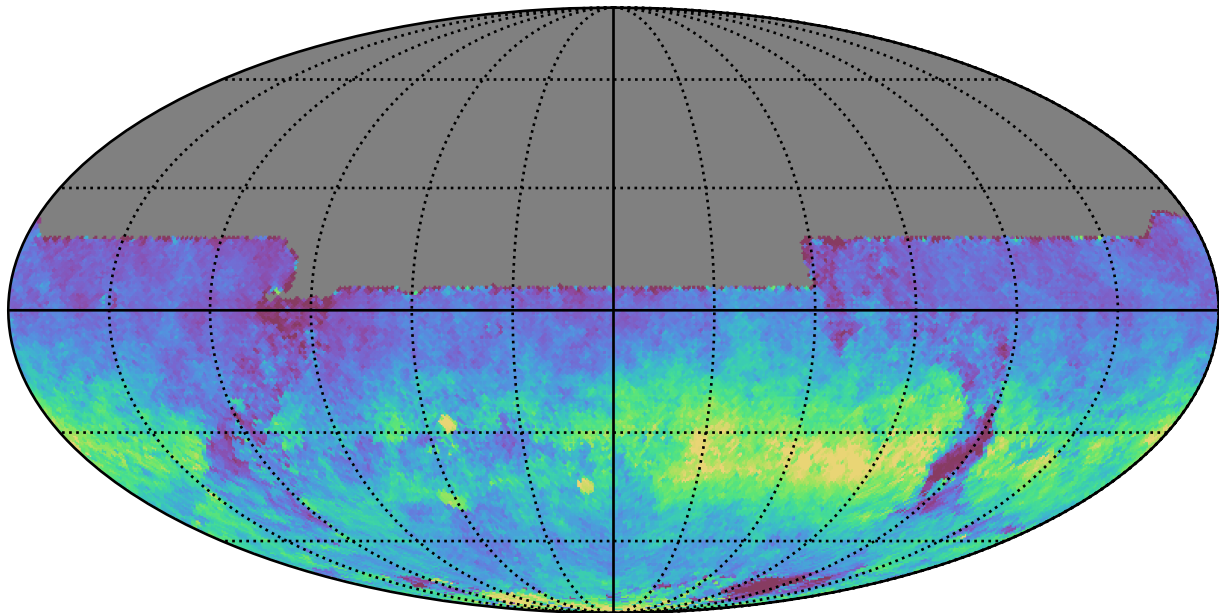
ddf_loaded_fl1_v3.4_10yrs All sky y band: AngleRms rotSkyPos
