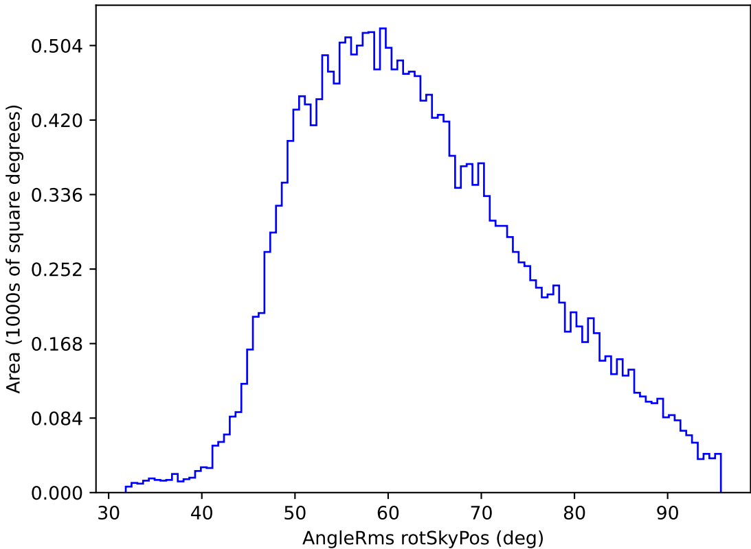
ddf_loaded_fl1_v3.4_10yrs All sky u band: AngleRms rotSkyPos
