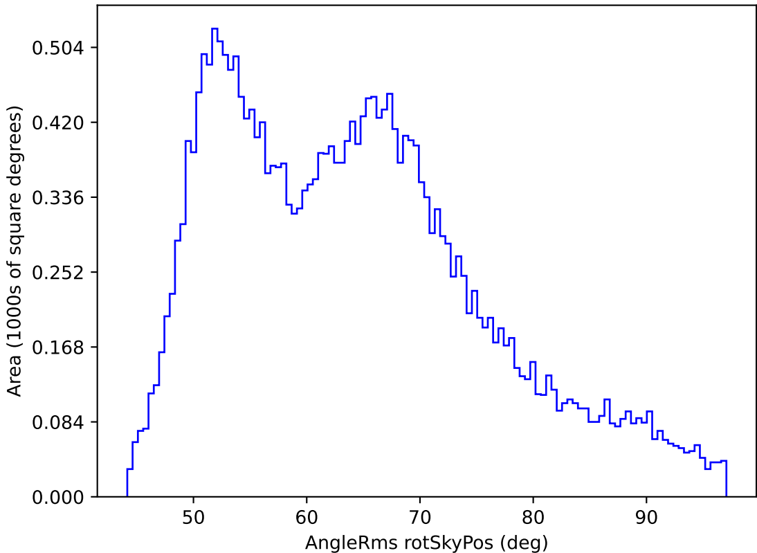
ddf_loaded_fl1_v3.4_10yrs All sky r band: AngleRms rotSkyPos
