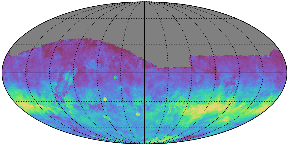
ddf_loaded_fl1_v3.4_10yrs All sky i band: AngleRms rotSkyPos
