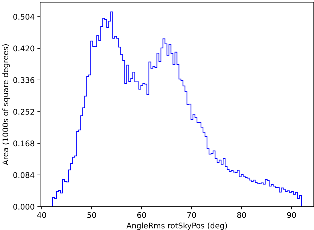
ddf_loaded_fl1_v3.4_10yrs All sky i band: AngleRms rotSkyPos
