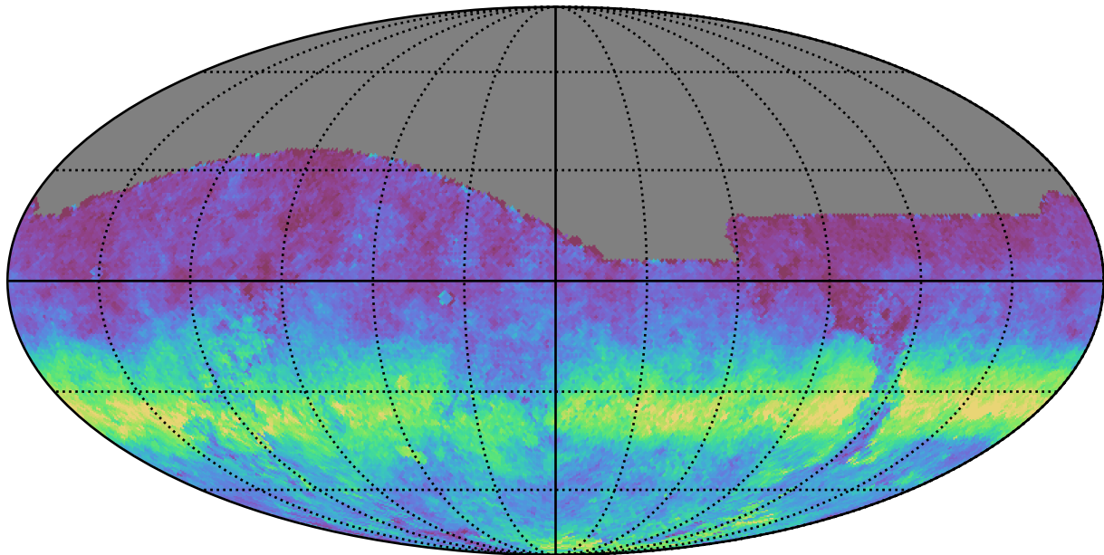
ddf_loaded_fl1_v3.4_10yrs All sky g band: AngleRms rotSkyPos
